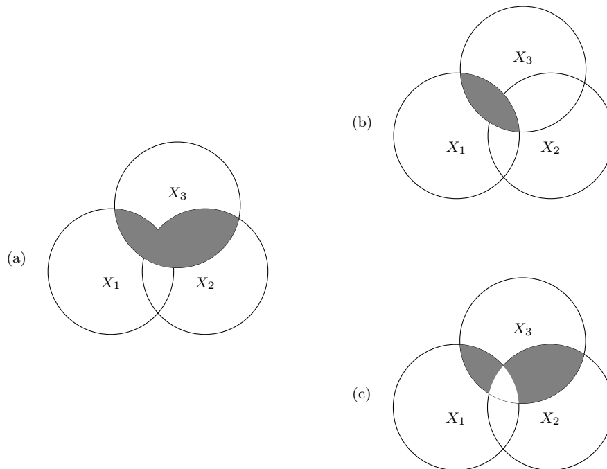
FIG 1. A network of three variables (variables are nodes) or the regression of node X_3 on the predictors X_1 and X_2 . Part (a) shows all variance that the predictors share with the dependent variable. Part (b) shows the contribution of X_1 to the explained variance in regression (i.e., R^2 ). Part (c) illustrates the variance that comes from each regressor separately. The shared variance is removed from the contribution of the regressors to prevent bias in the associated coefficients.
