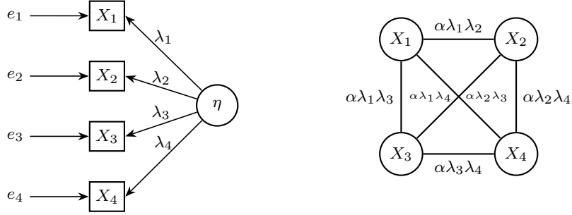
FIG 2. The left panel shows a unidimensional latent variable model with observed variables X_1, X_2, X_3 and X_4 , a scalar latent variable \eta , and loadings \lambda_1, \lambda_2, \lambda_3 and \lambda_4 . The e_i on the left are the error terms for the observed variables. The right panel shows the associated network model. All observed variables are connected to each other with parameter \alpha\lambda_i\lambda_j , where -\alpha^{-1} = \lambda^T\lambda + 1 (see (8) and further for details on the weights)
